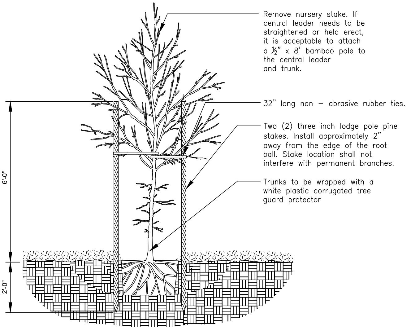
SECTION VIEW
