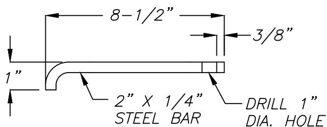
LOCKING BAR
